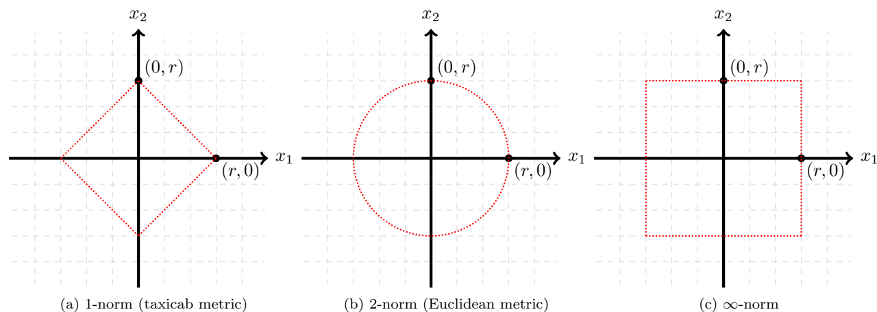
Figure 1: B_r(0) for different metrics
